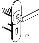
DIN 0241 Outside single handle (with inside panic bar)
